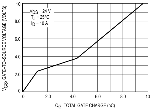
Figure 5. Gate Charge
