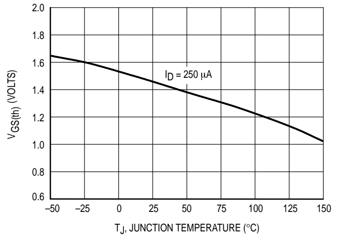
Figure 10. Threshold Voltage
