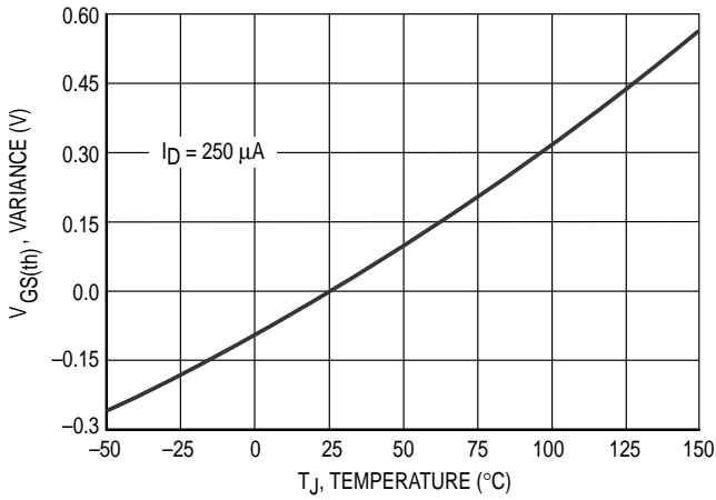
Figure 9. Threshold Voltage
