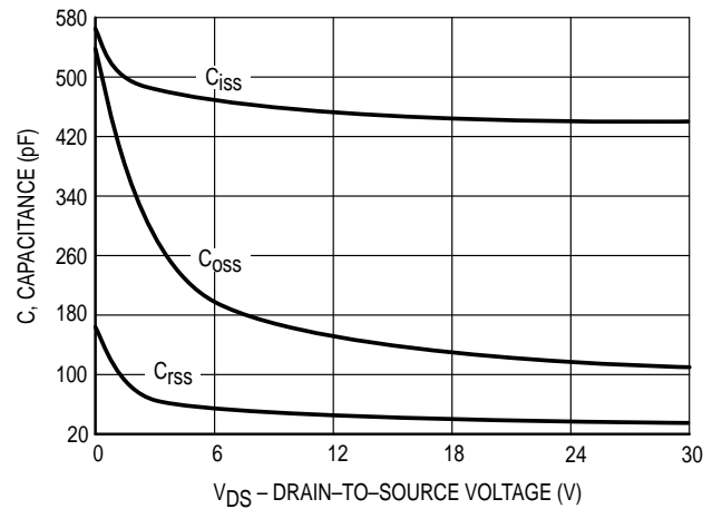
Figure 4. Capacitance
