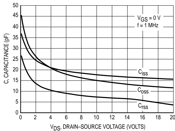
Figure 7. Capacitance Variation
