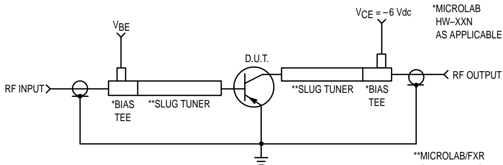
Figure 3. Functional Circuit Schematic
