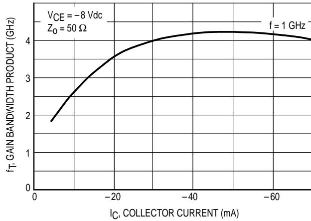
Figure 8. Gain-Bandwidth Product versus Current
