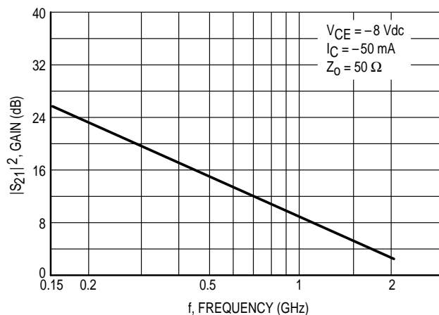
Figure 14. Insertion Gain versus Frequency
