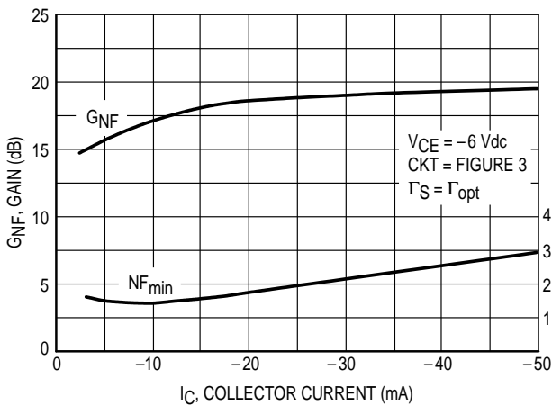
Figure 11. Tuned Circuit — Frequency 500 MHz
