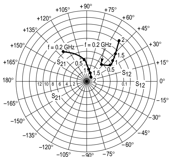
Figure 31. Forward/Reverse Transmission Coefficients versus Frequency (GHz) VCE = 6.0 V, IC = 5.0 mA
