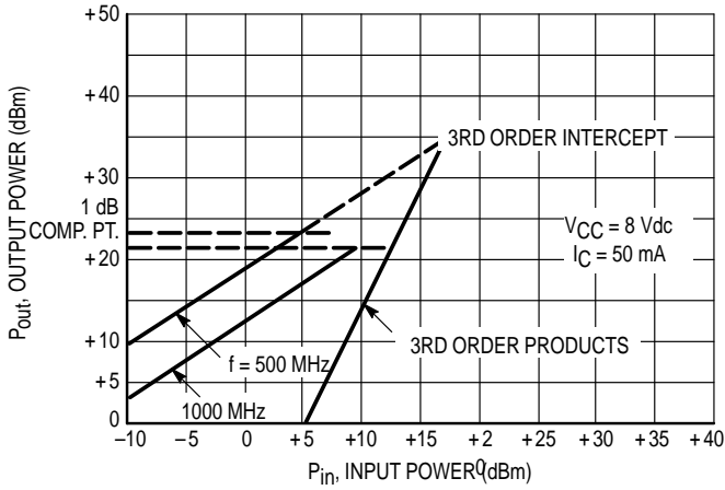
Figure 28. 1.0 dB Compression Point and Third Order Intercept
