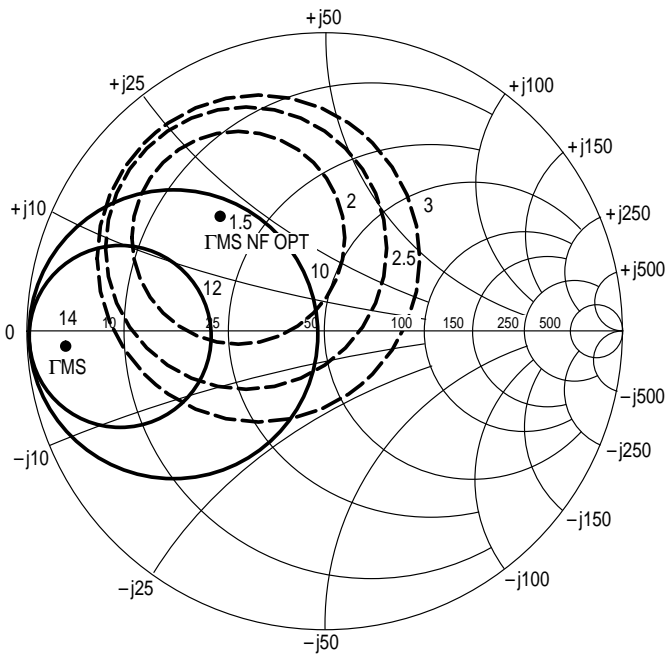
Figure 32. MRF571 Constant Gain and Noise Figure Contours
