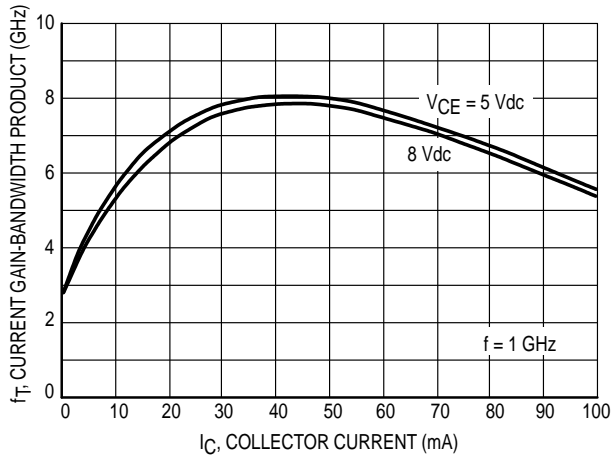
Figure 26. f_T , Current Gain–Bandwidth Product versus Collector Current
