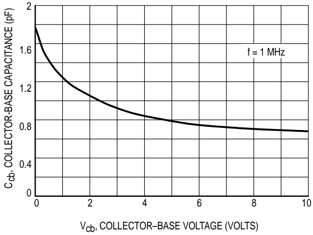
Figure 9. Collector-Base Capacitance versus Collector-Base Voltage
