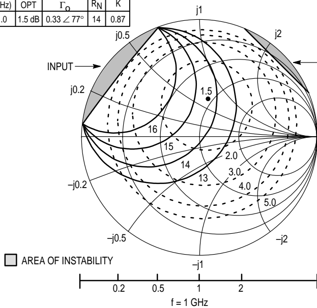
Figure 23. MRF947 Series Constant Gain and Noise Figure Contours
