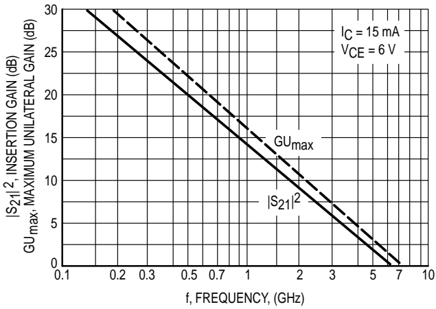
Figure 5. MMR941LT1, T3
