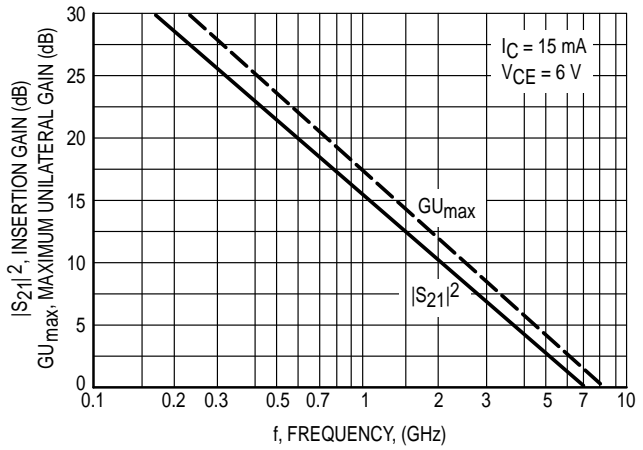
Figure 6. MRF9411LT1
