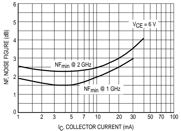
Figure 8. Minimum Noise Figure versus Collector Current
