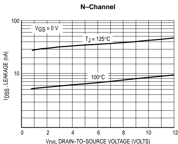
Figure 6. Drain-To-Source Leakage Current versus Voltage
