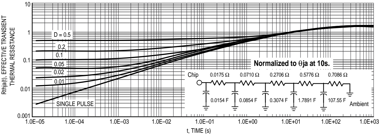
Figure 13. Thermal Response
