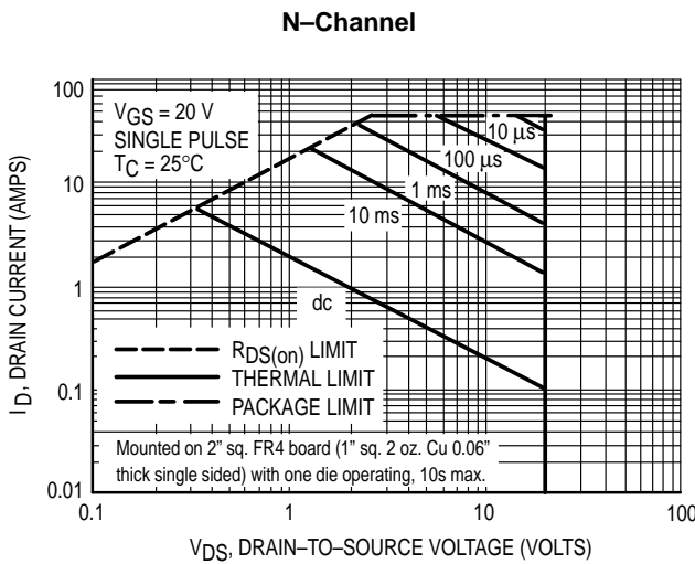
Figure 12. Maximum Rated Forward Biased Safe Operating Area
