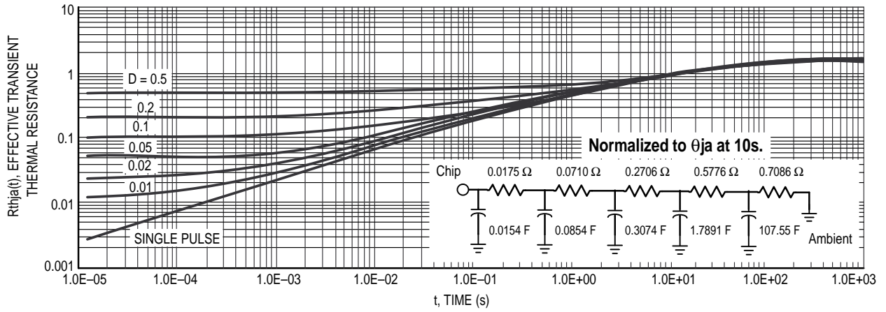
Figure 10. Thermal Response
