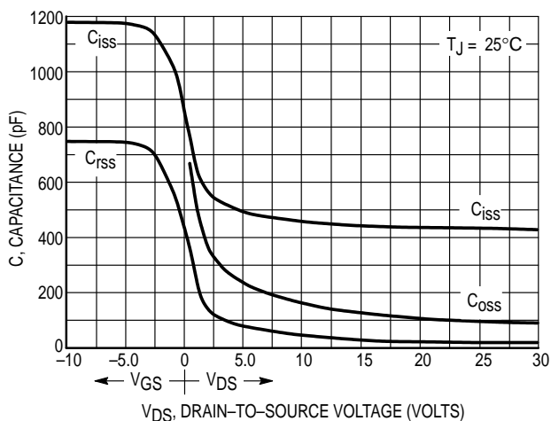
Figure 8. Capacitance Variation
