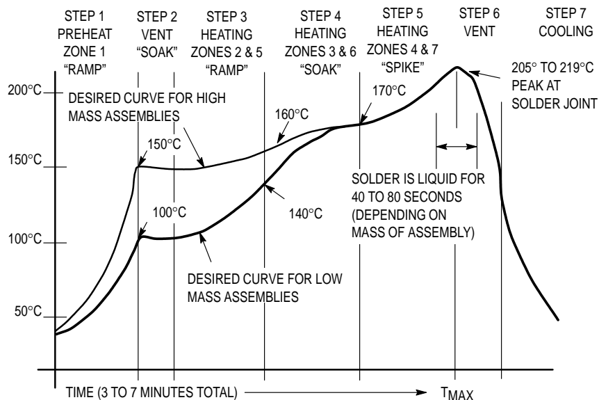
Figure 16. Typical Solder Heating Profile
