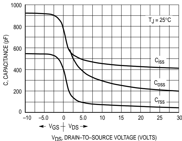
Figure 7. Capacitance Variation
