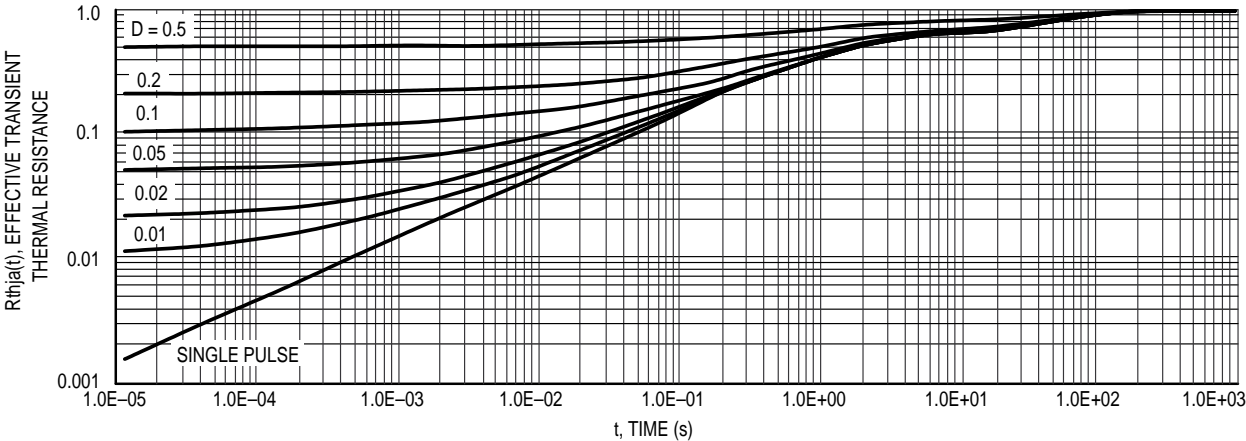
Figure 14. Thermal Response
