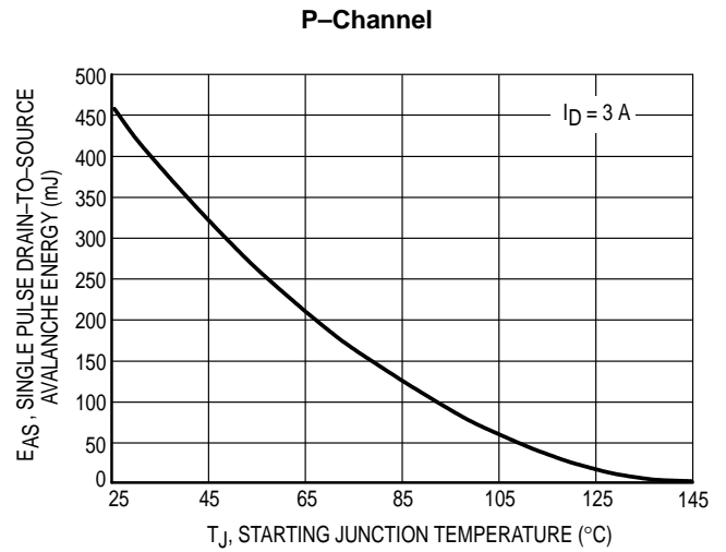
Figure 13. Maximum Avalanche Energy versus Starting Junction Temperature
