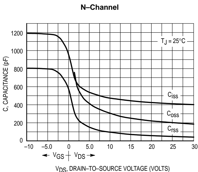
Figure 7. Capacitance Variation
