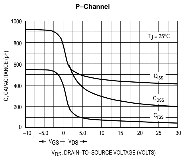
Figure 7. Capacitance Variation
