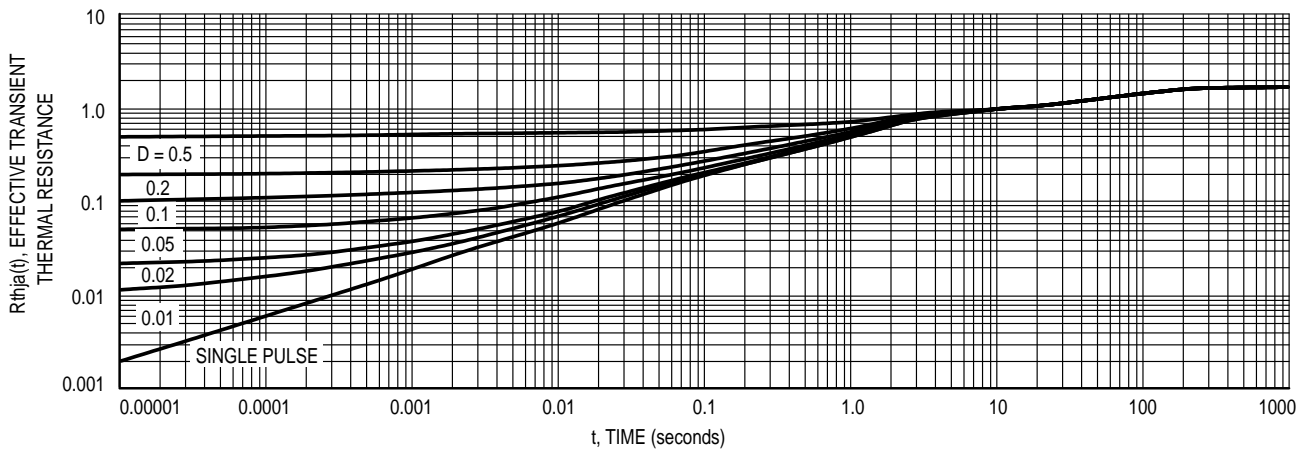
Figure 14. Thermal Response
