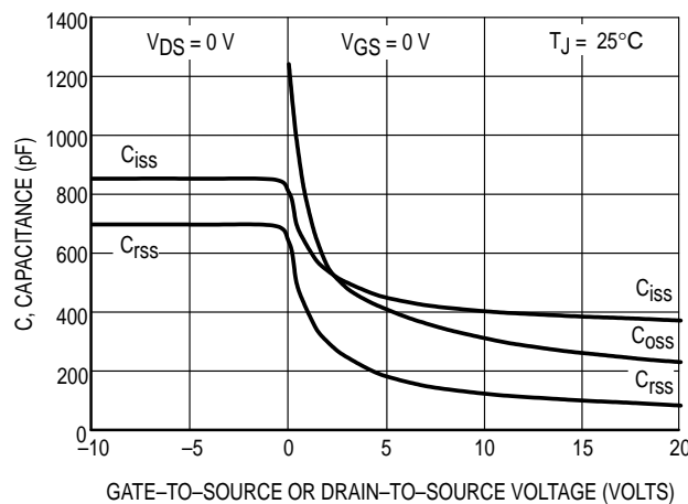
Figure 7. Capacitance Variation
