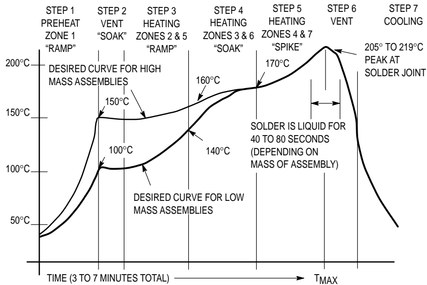
Figure 15. Typical Solder Heating Profile
