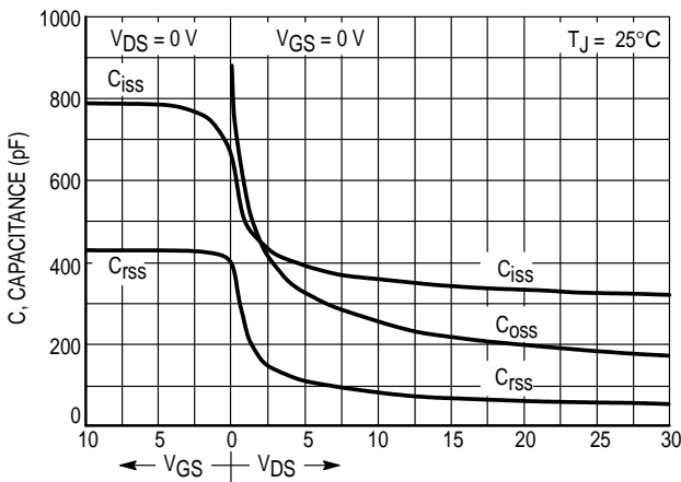
Figure 7. Capacitance Variation
