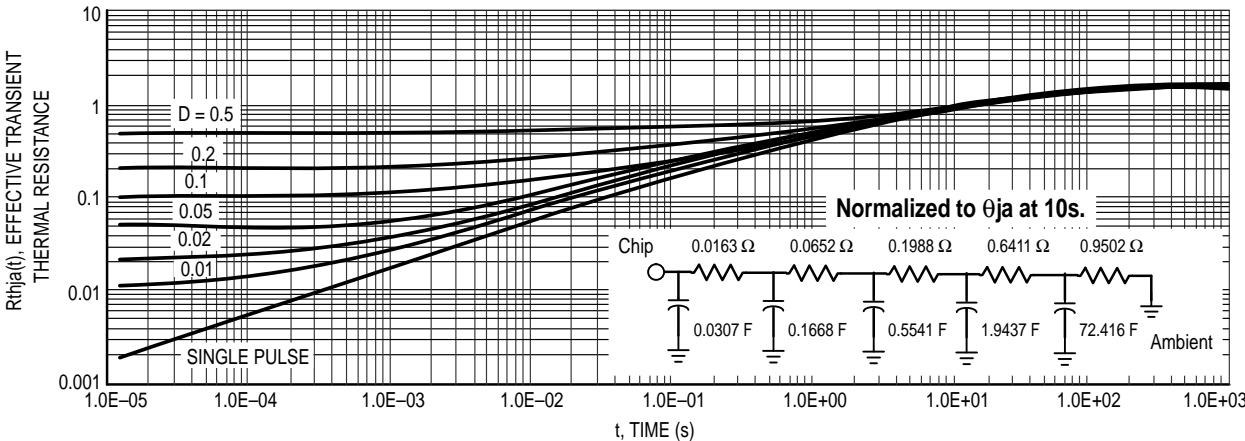
Figure 13. Thermal Response
