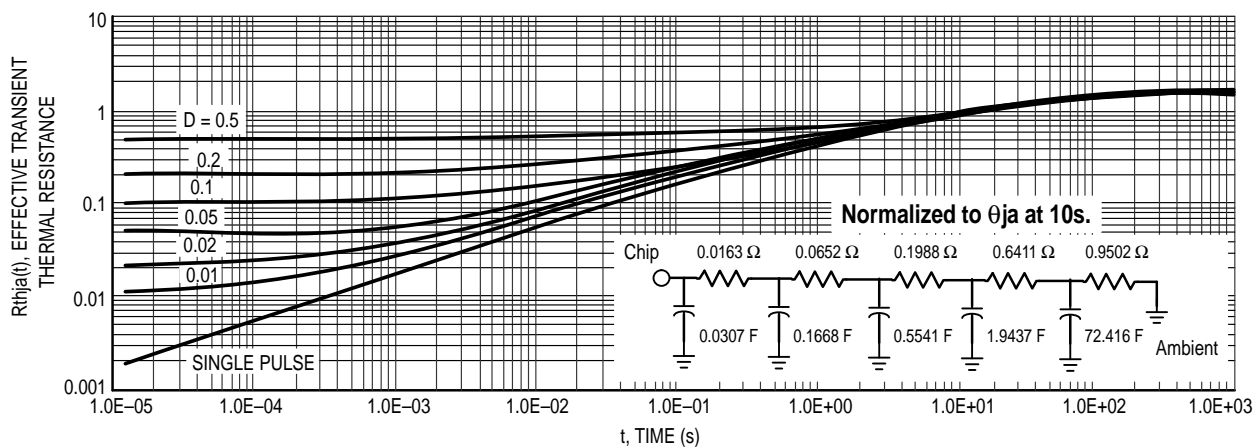
Figure 14. Thermal Response
