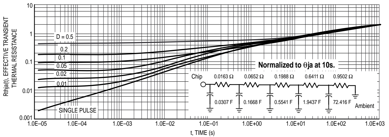
Figure 14. Thermal Response
