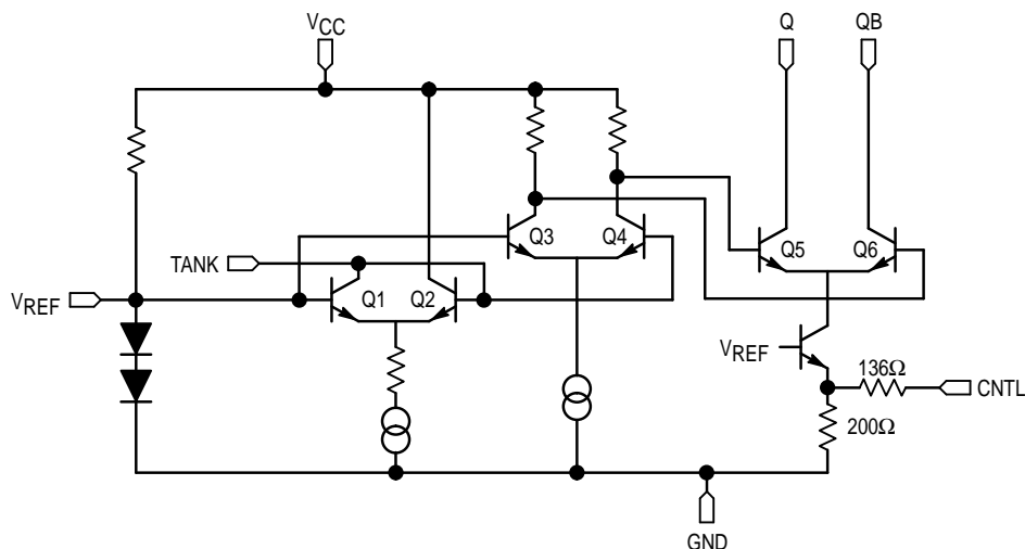
Figure 1. Simplified Schematic
