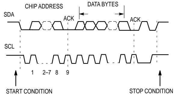
Figure 2. M_BUS Format
