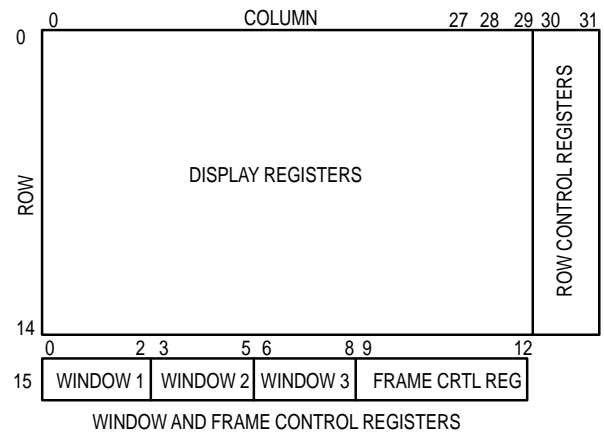
Figure 5. Memory Map
