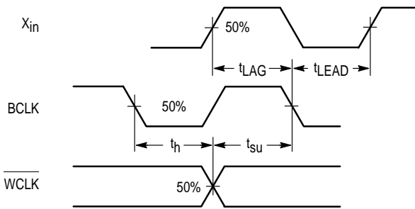
Figure 6. WCLK Timing (DMODE = 1, WDLY = 1)
