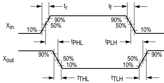
Figure 1. X out Propagation Delay Timing
