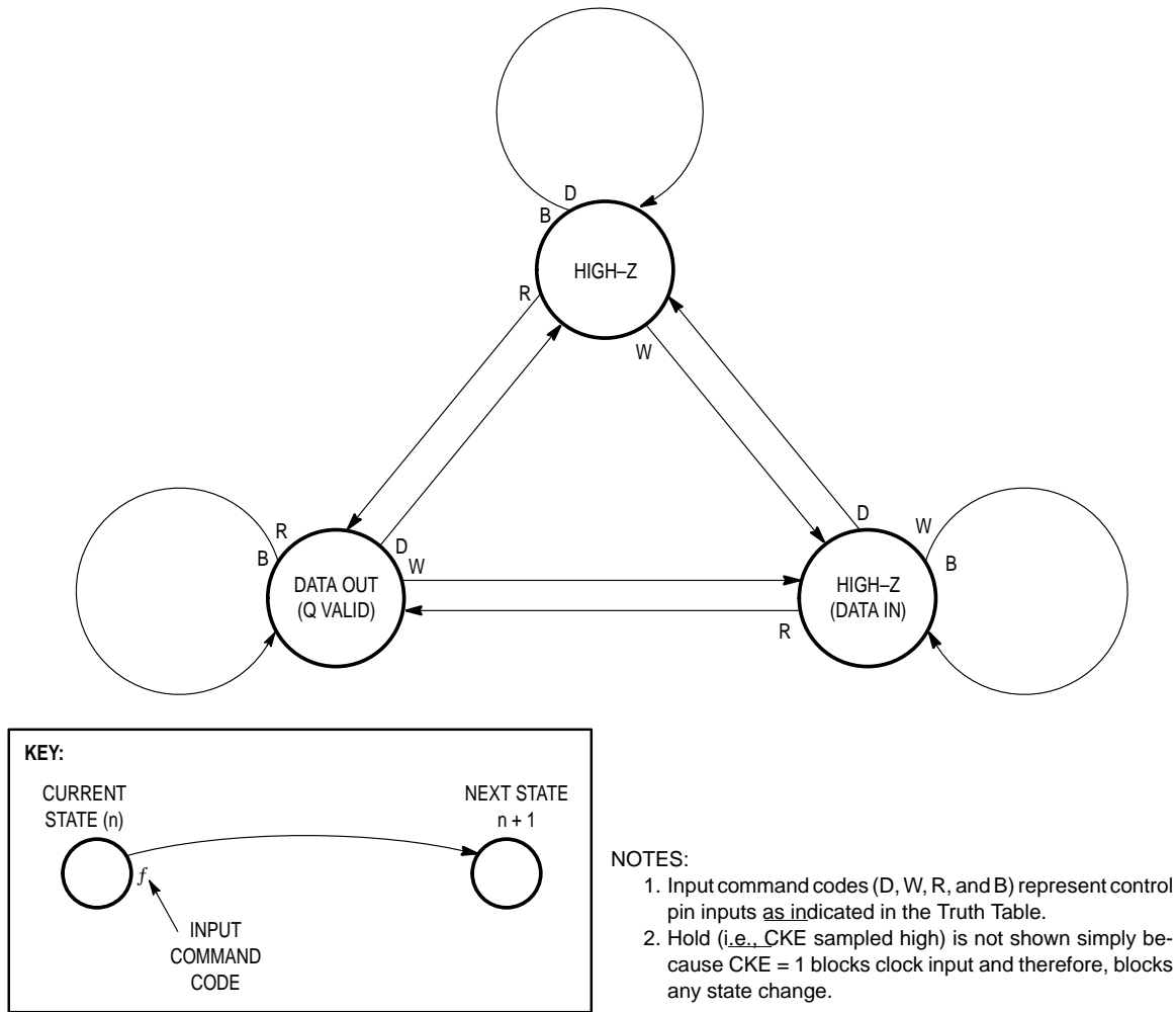
Figure 3. Data I/O State Diagram
