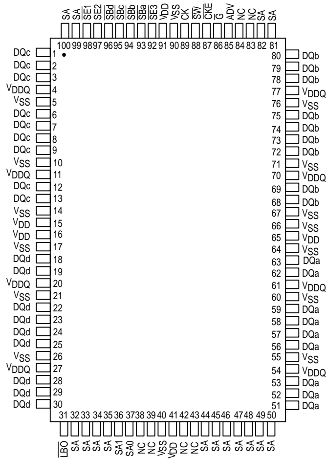
TOP VIEW MCM63Z737
