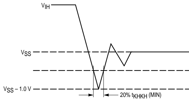
Figure 5. Undershoot Voltage
