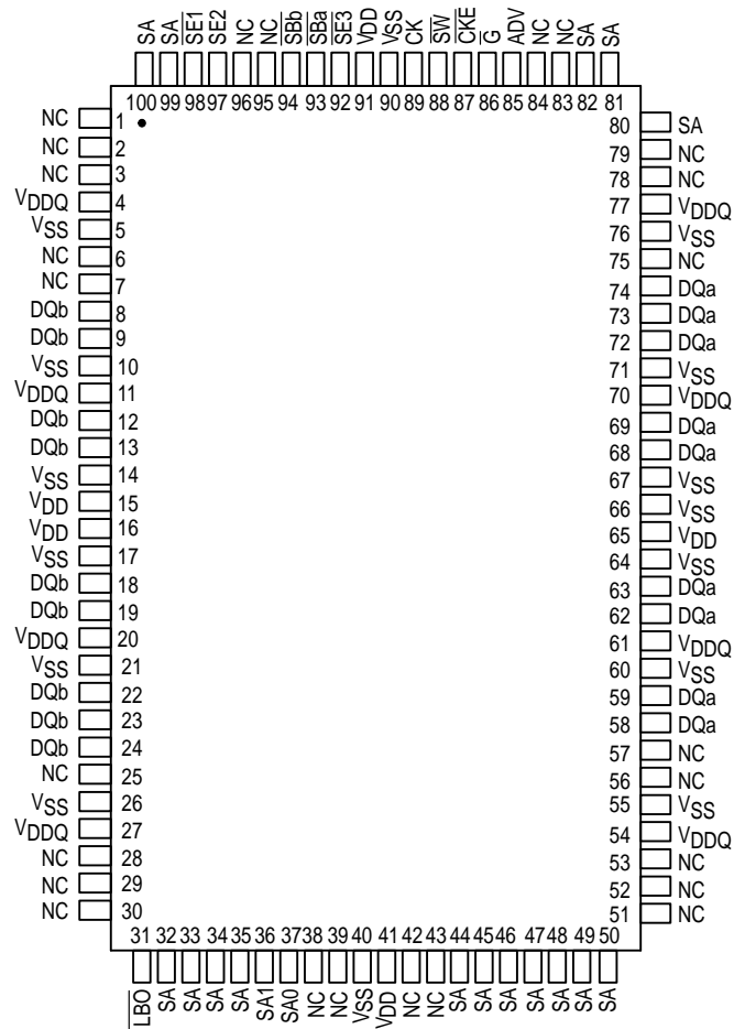
TOP VIEW MCM63Z819
