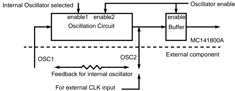
Figure 8. Oscillator Circuitry
