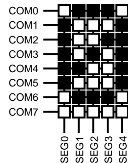
Figure 9a. LCD Display Example "0"
