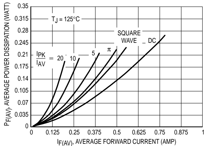
Figure 6. Power Dissipation
