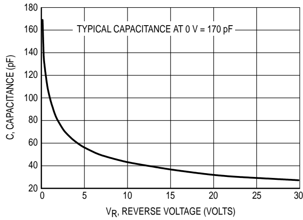
Figure 3. Typical Capacitance
