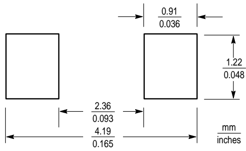
SOD-123
