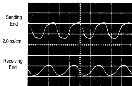
FIGURE 2 — 400 MBS WAVEFORMS
