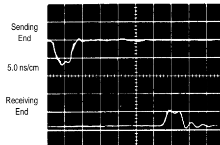
FIGURE 3 — PULSE PROPAGATION WAVEFORMS
