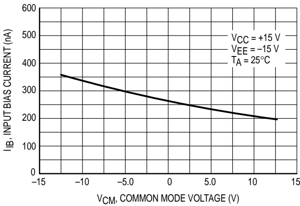
Figure 5. Input Bias Current versus Common Mode Voltage
