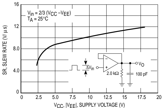
Figure 23. Slew Rate versus Supply Voltage
