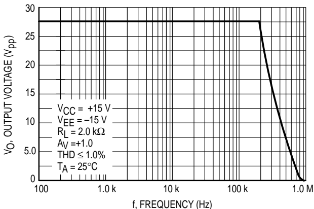
Figure 15. Output Voltage versus Frequency
