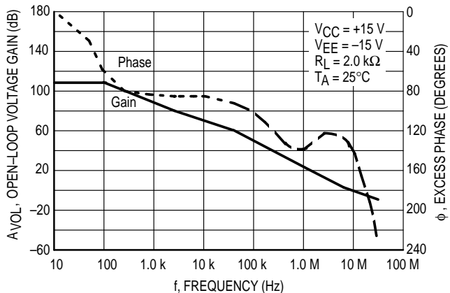
Figure 25. Voltage Gain and Phase versus Frequency
