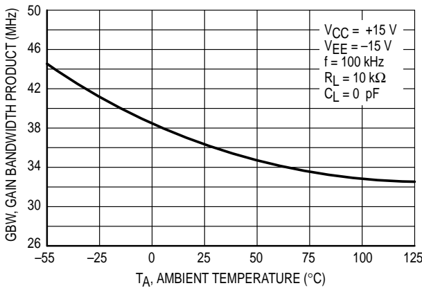
Figure 13. Gain Bandwidth Product versus Temperature
