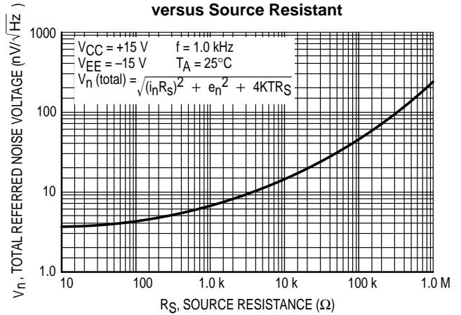
Figure 30. Total Input Referred Noise Voltage versus Source Resistor
