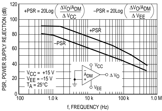
Figure 11. Power Supply Rejection versus Frequency
