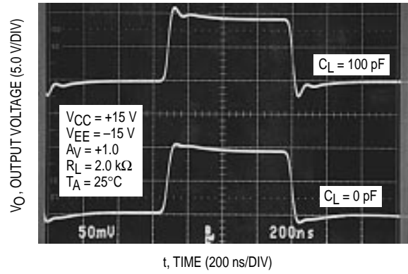
Figure 34. Noninverting Amplifier Overshoot
