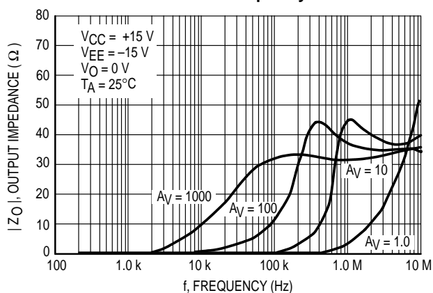
Figure 18. Output Impedance versus Frequency
