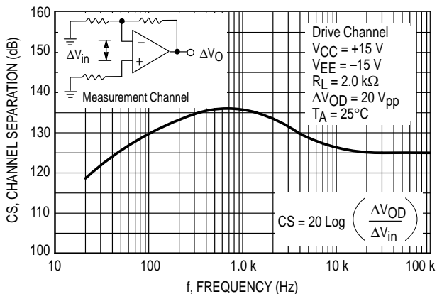
Figure 19. Channel Separation versus Frequency
