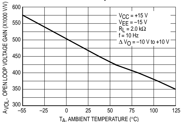
Figure 17. Open Loop Voltage Gain versus Temperature
