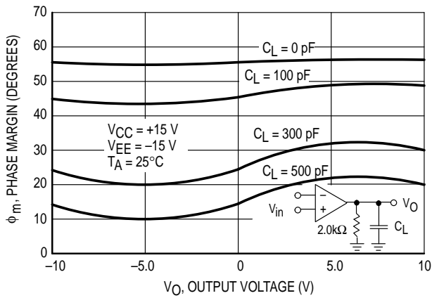
Figure 27. Phase Margin versus Output Voltage
