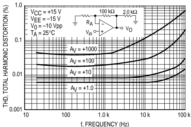
Figure 21. Total Harmonic Distortion versus Frequency
