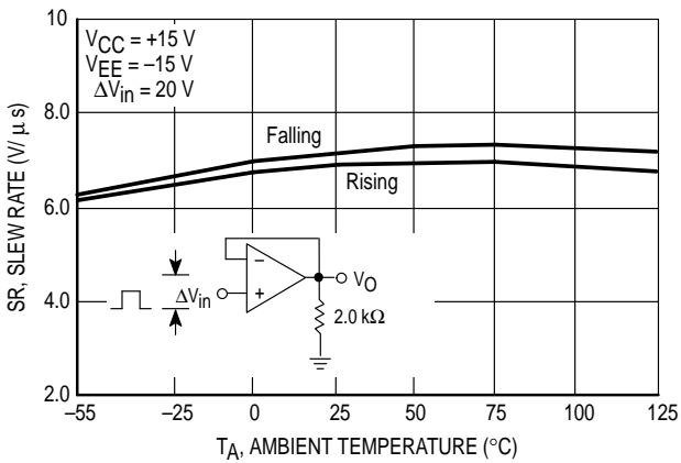
Figure 23. Slew Rate versus Temperature
