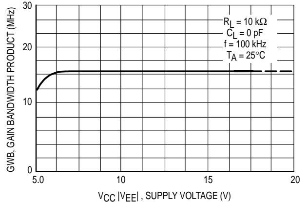
Figure 12. Gain Bandwidth Product versus Supply Voltage
