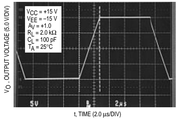
Figure 31. Noninverting Amplifier Slew Rate
