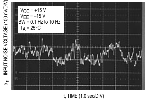
Figure 33. Low Frequency Noise Voltage versus Time
