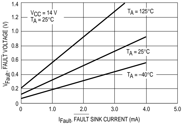
Figure 6. Fault Voltage versus Fault Sink Current
