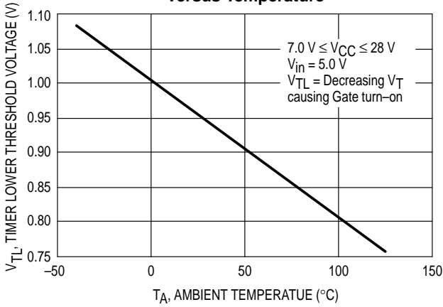
Figure 12. Timer Lower Threshold Voltage versus Temperature
