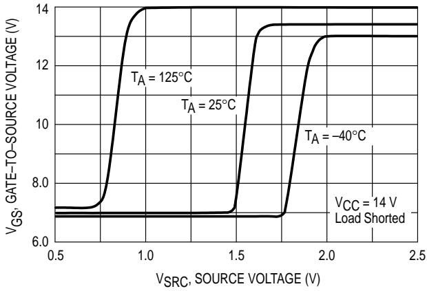
Figure 18. Gate-to-Source Voltage versus Source Voltage
