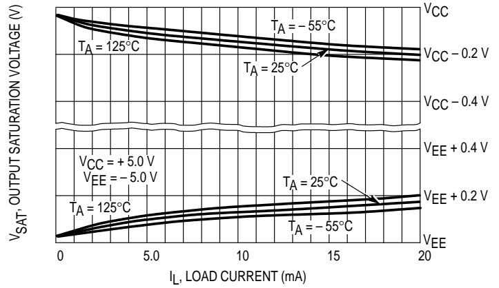
Figure 9. Output Saturation Voltage versus Load Current
