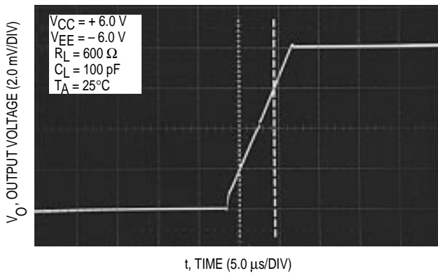
Figure 26. Noninverting Amplifier Slew Rate
