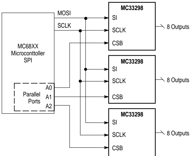
Figure 13. Parallel Input SPI Control
