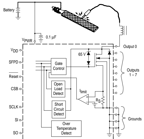
Figure 24. Transient Latch-Up Immunity File Test
