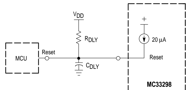
Figure 15. Power "On" Reset
