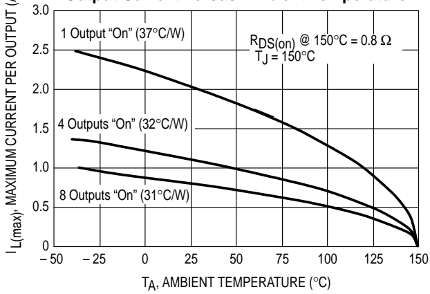
Figure 21. Maximum DIP Package Steady State Output Current versus Ambient Temperature
