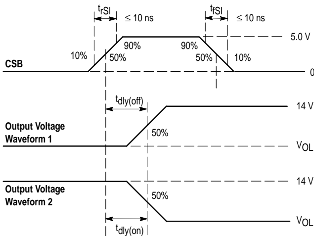
Figure 9. Turn-On/Off Waveforms
