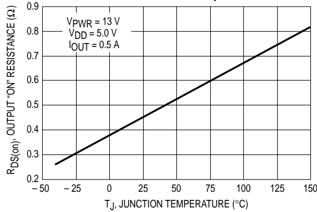
Figure 23. Maximum Output "On" Resistance versus Junction Temperature
