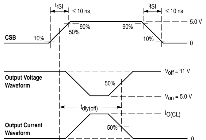
Figure 10. Output Fault Unlatch Disable Delay Waveforms
