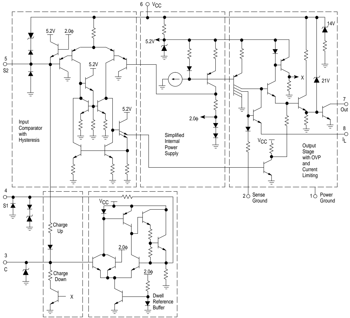
Figure 3. Internal Schematic
