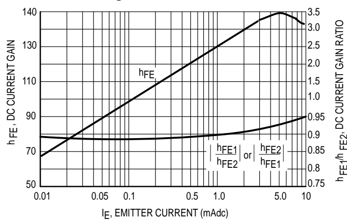
Figure 5. DC Current Gain
