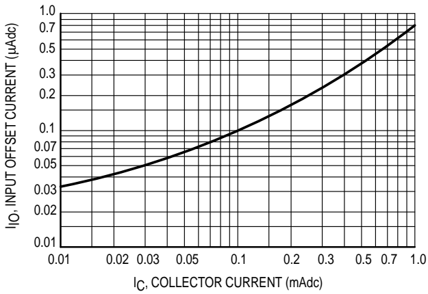
Figure 3. Input Offset Characteristics for Q1 and Q2
