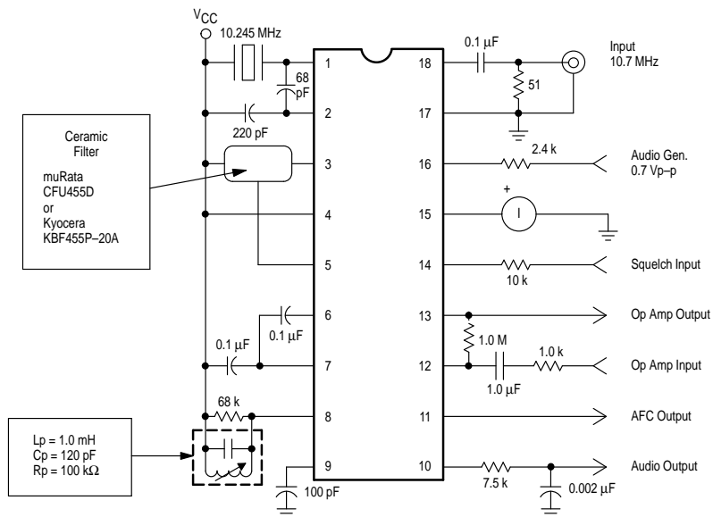
Figure 3. Test Circuit
