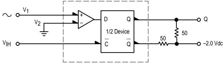
(A) TEST CIRCUIT
