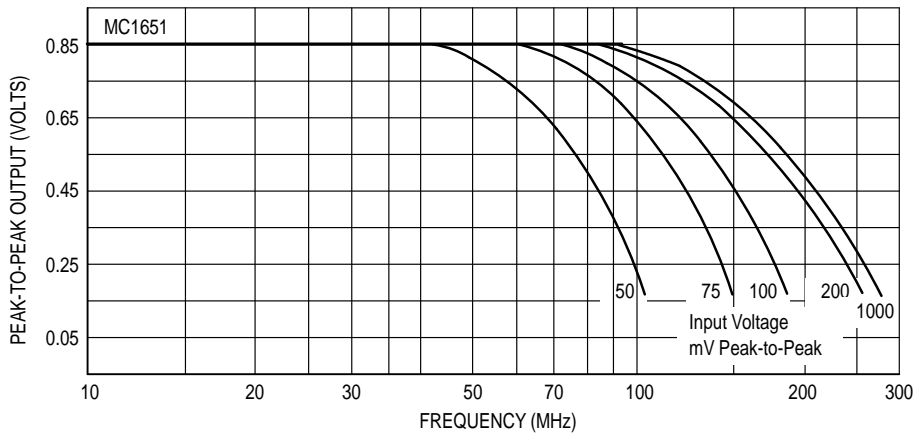
(B) TYPICAL OUTPUT LOGIC SWING versus FREQUENCY
