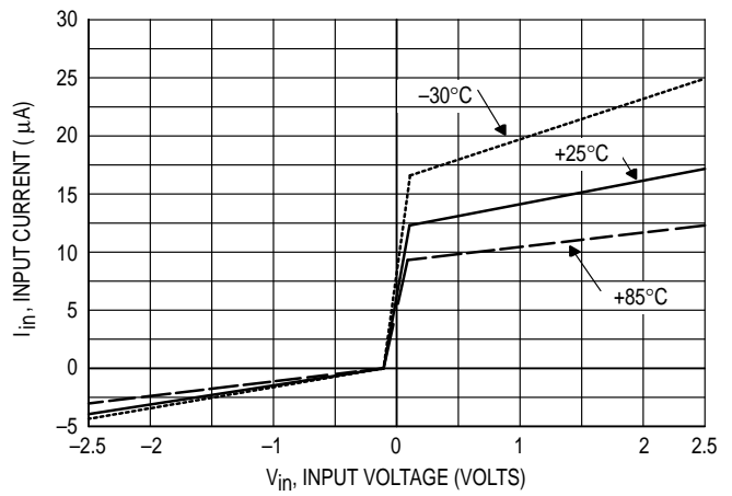
Typical MC1651 (Complementary Input Grounded)
