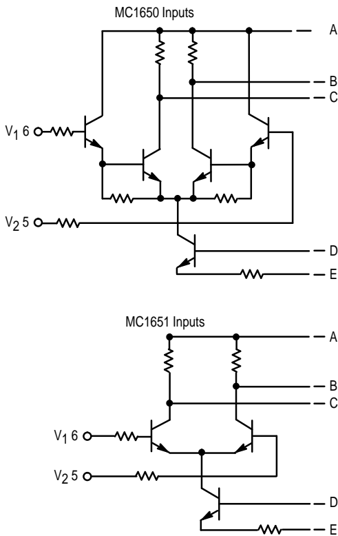
CIRCUIT SCHEMATIC 1/2 of Device Shown
