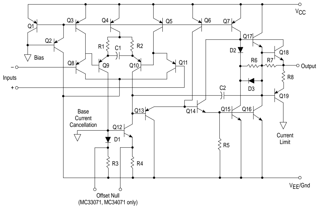
Representative Schematic Diagram (Each Amplifier)
