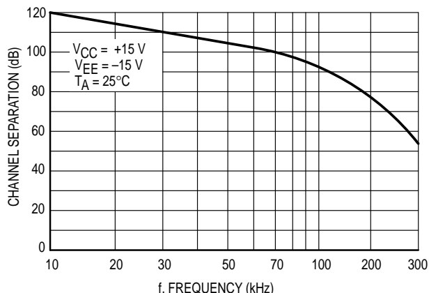
Figure 35. Channel Separation versus Frequency
