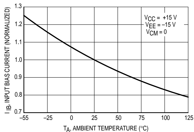
Figure 6. Normalized Input Bias Current versus Temperature
