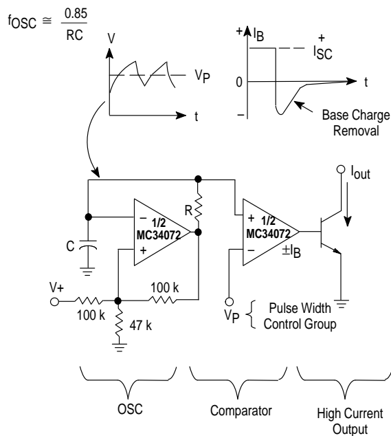
Figure 54. High Frequency Pulse Width Modulation
