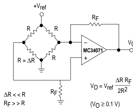
Figure 52. Bridge Current Amplifier
