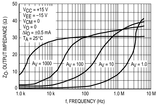
Figure 13. Output Impedance versus Frequency
