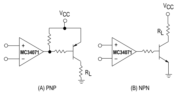
Figure 46. Transistor Driver
