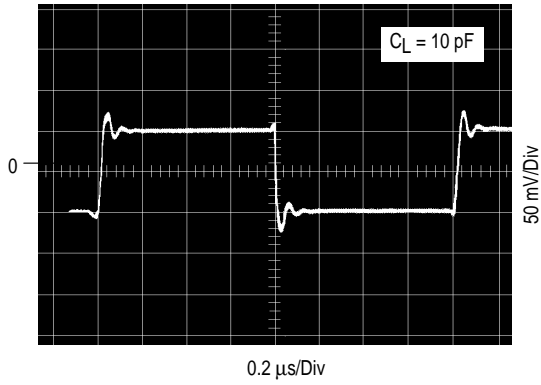
Figure 24. Small Signal
