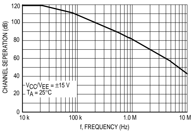
Figure 32. Channel Separation versus Frequency
