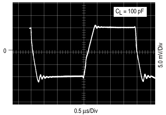
Figure 27. Large Signal
