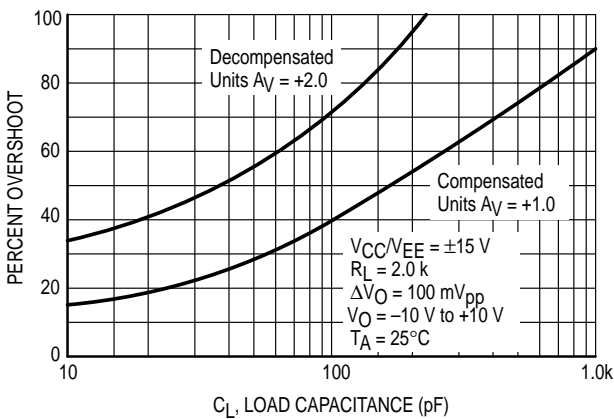
Figure 18. Percent Overshoot versus Load Capacitance
