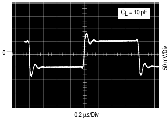
Figure 26. Small Signal
