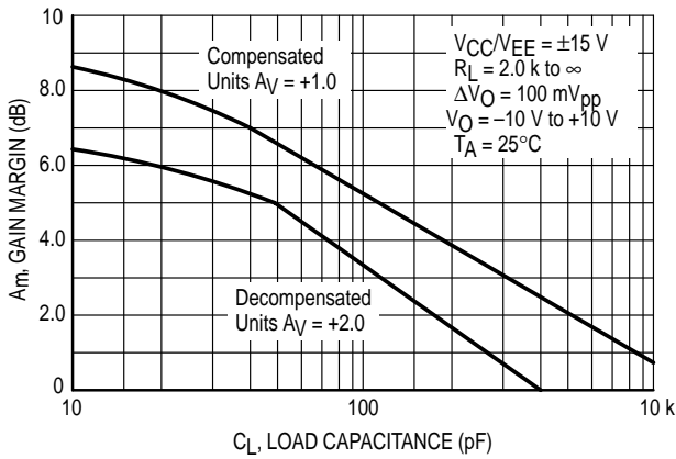
Figure 20. Gain Margin versus Load Capacitance
