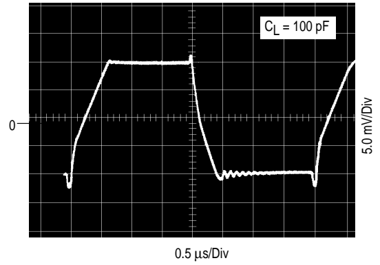
Figure 25. Large Signal
