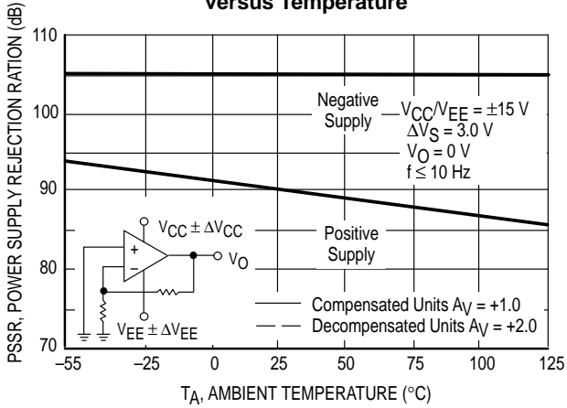
Figure 30. Power Supply Rejection Ratio versus Temperature
