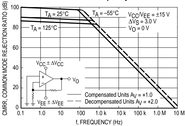
Figure 28. Common Mode Rejection Ratio versus Frequency
