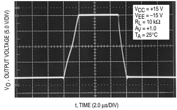
Figure 28. Transient Response
