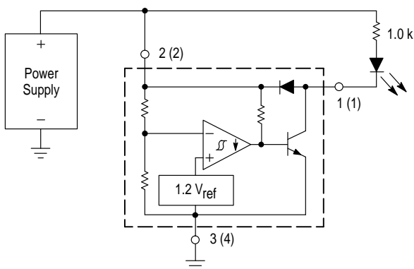
Figure 15. Voltage Monitor
