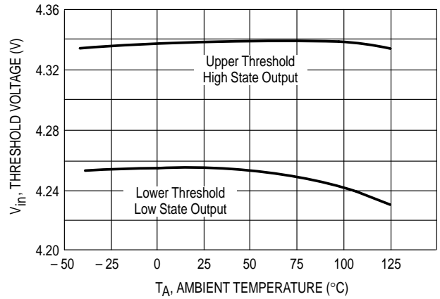
Figure 6. MC3X164-5 Comparator Threshold Voltage versus Temperature
