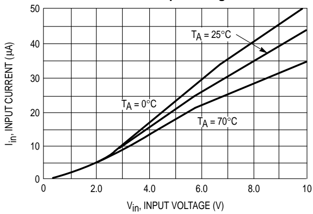
Figure 7. MC3X164-3 Input Current versus Input Voltage
