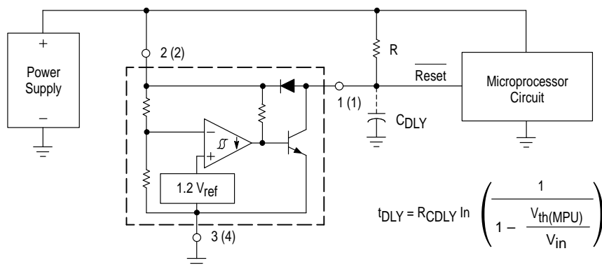
Figure 13. Low Voltage Microprocessor Reset
