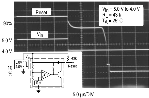
Figure 12. Reset Delay Time (MC3X164–5 Shown)
