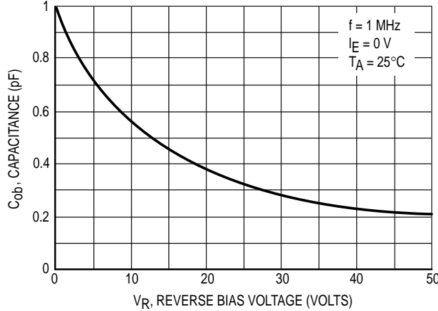
Figure 29. Output Capacitance
