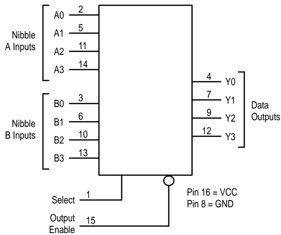
Pinout: 16-Lead Plastic Package (Top View)
