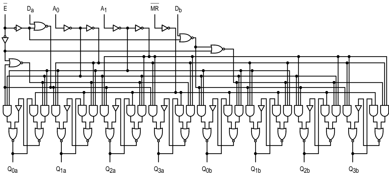
LOGIC DIAGRAM
