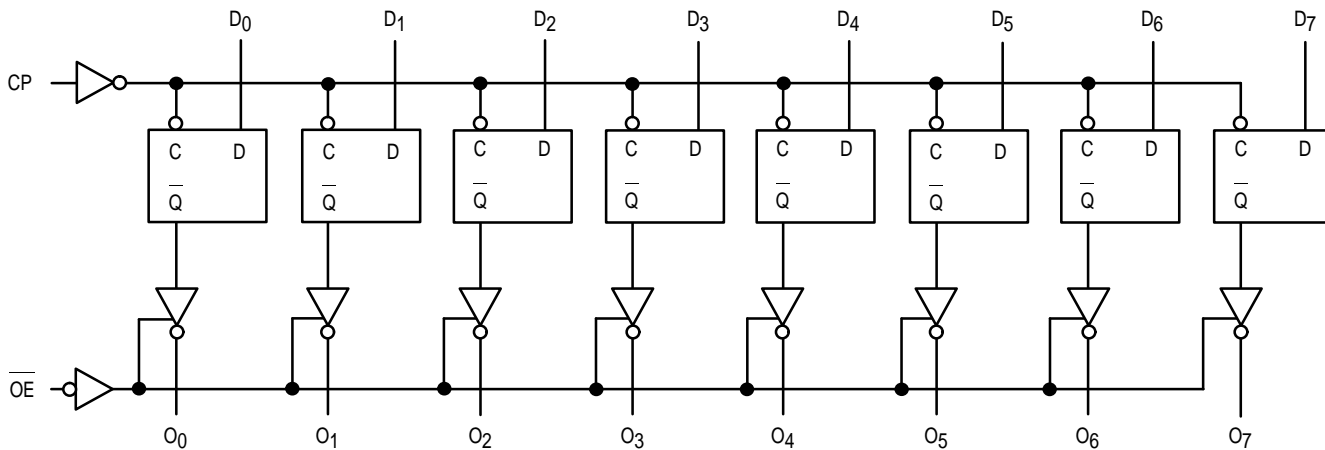
LOGIC DIAGRAM
