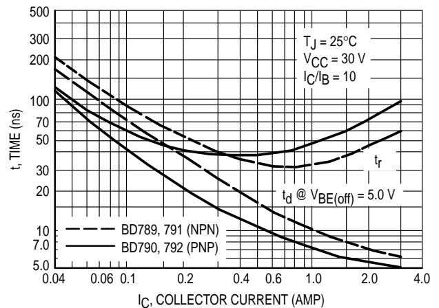
Figure 3. Turn-On Time
