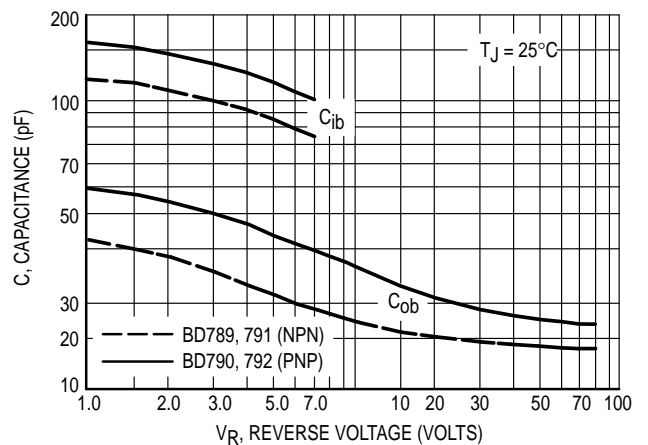
Figure 7. Capacitance
