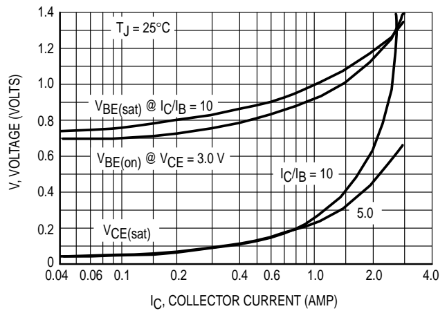
Figure 9. "On" Voltages
