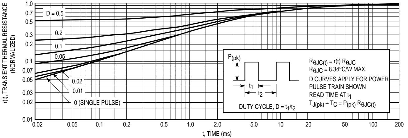
Figure 4. Thermal Response
