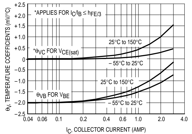
Figure 10. Temperature Coefficients
