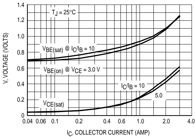
Figure 9. "On" Voltages
