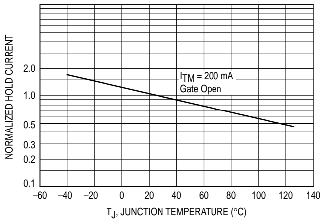
FIGURE 5 – HOLD CURRENT
