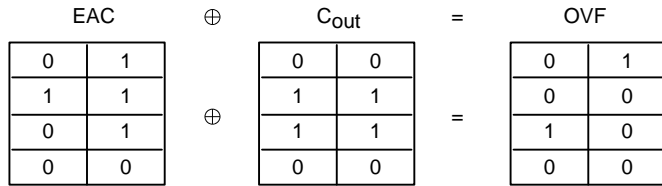
Figure 10. Mapping of EAC, Sign and Overflow Logic
