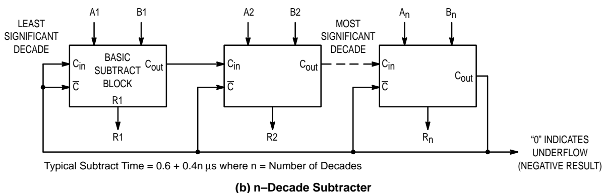
Figure 6. Subtraction of Unsigned NBCD Numbers
