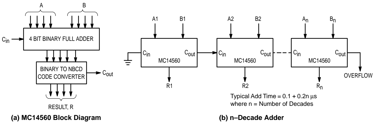
Figure 5. Addition of Unsigned NBCD Numbers
