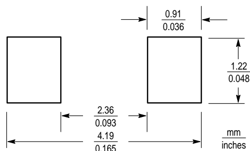
SOD-123
