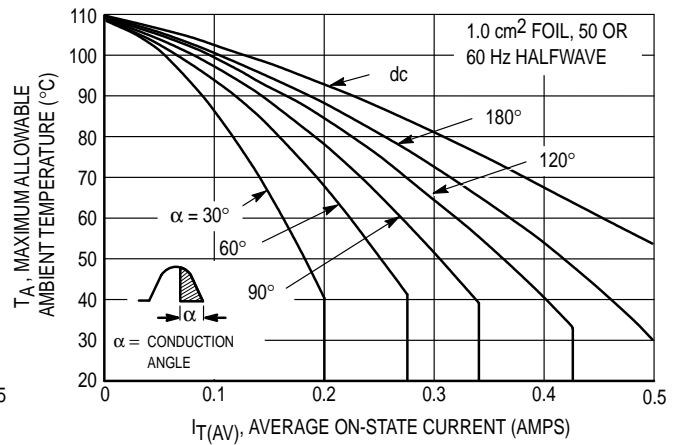
Figure 5. Current Derating, 1.0\text{ cm}^2 Pad Reference: Ambient Temperature
