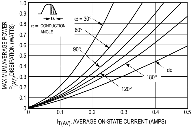
Figure 8. Power Dissipation
