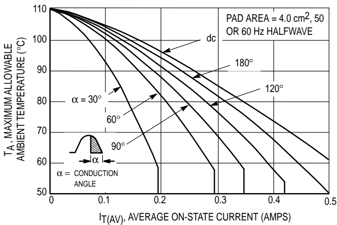
Figure 6. Current Derating, 2.0\text{ cm}^2 Pad Reference: Ambient Temperature
