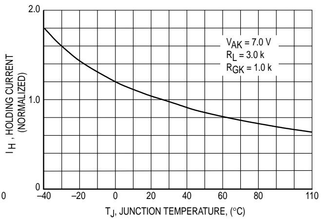
Figure 11. Typical Normalized Holding Current versus Junction Temperature
