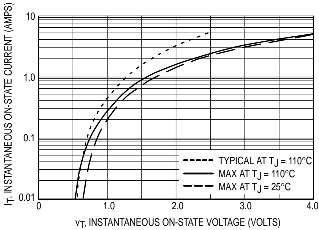
Figure 2. On-State Characteristics
