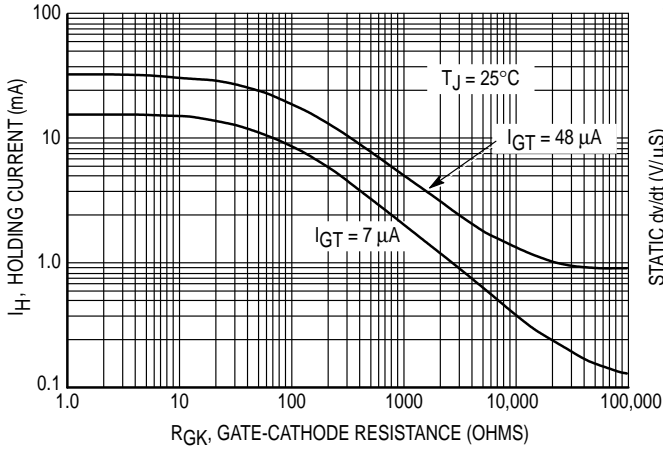
Figure 14. Holding Current Range versus Gate-Cathode Resistance
