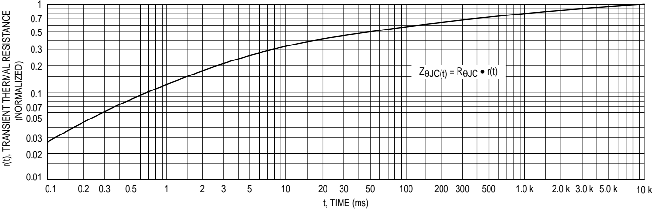
Figure 6. Thermal Response
