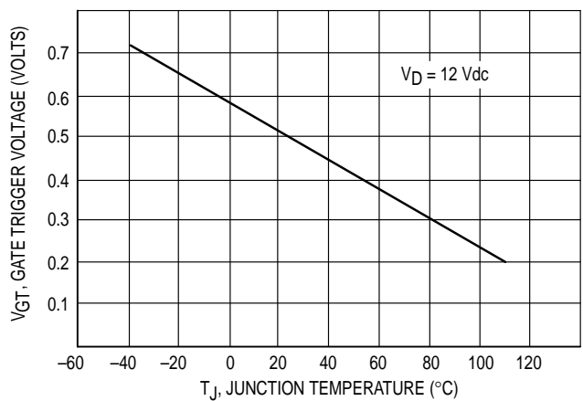
Figure 4. Gate Voltage
